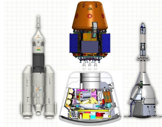
HUMAN RATED LVM 4-GAGANYAAN-PAD ABORT SYSTEM
